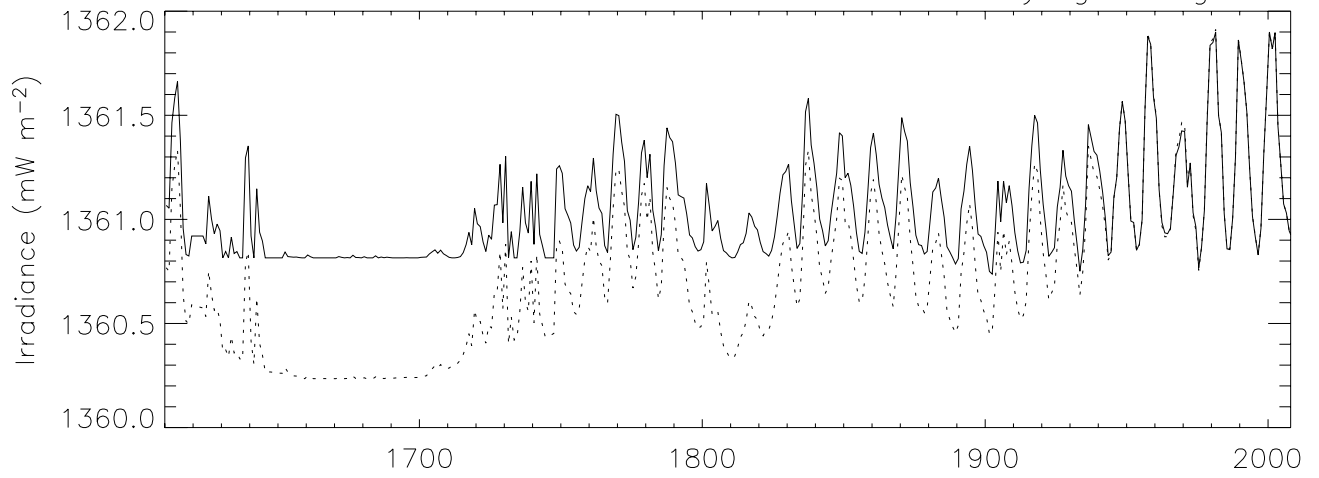
Total Solar Irradiance scaled with and without varying background
